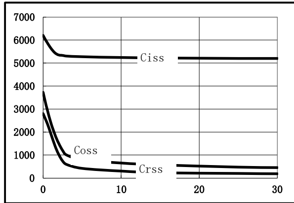
Fig.2 Capacitance Characteristics
